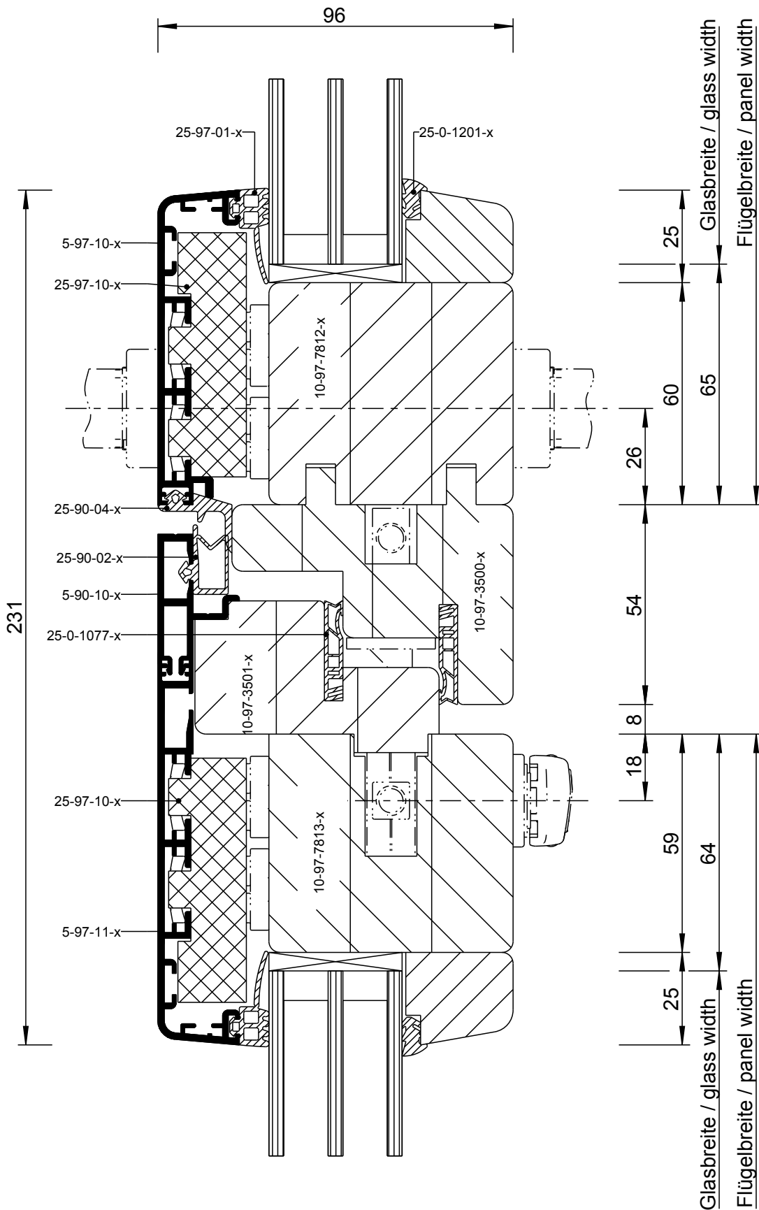
Detail 97-8-2
