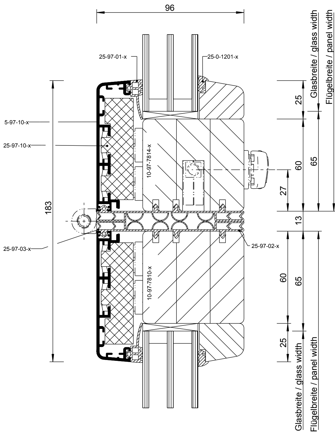
Detail 97-7-2
