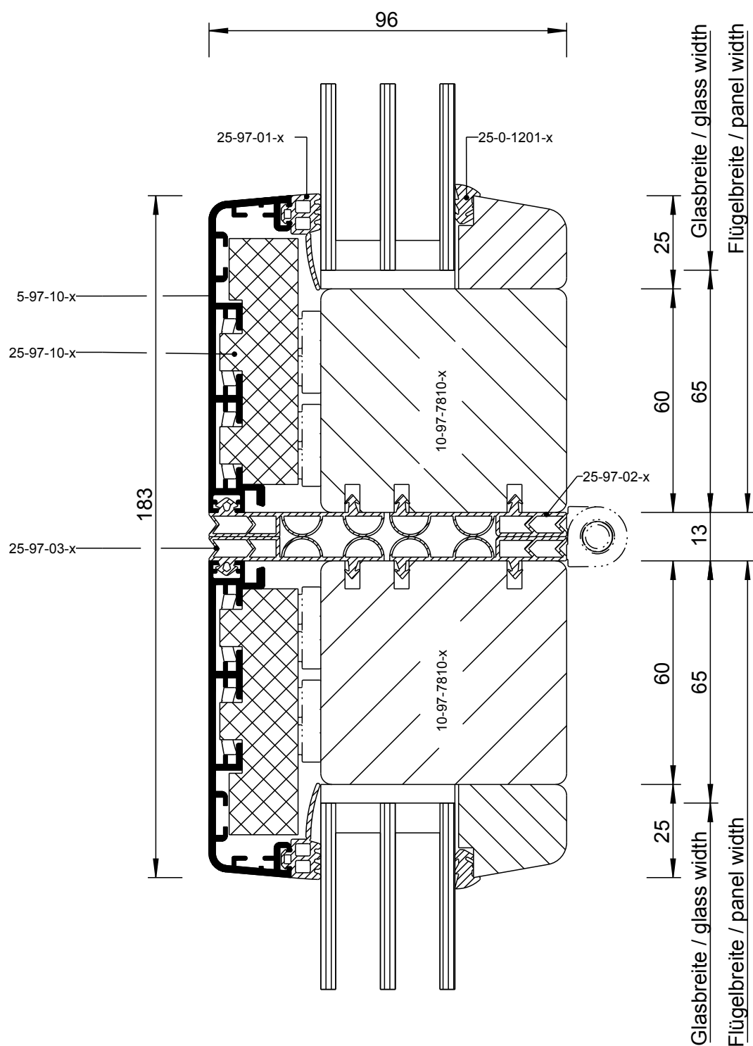
Detail 97-7-0
