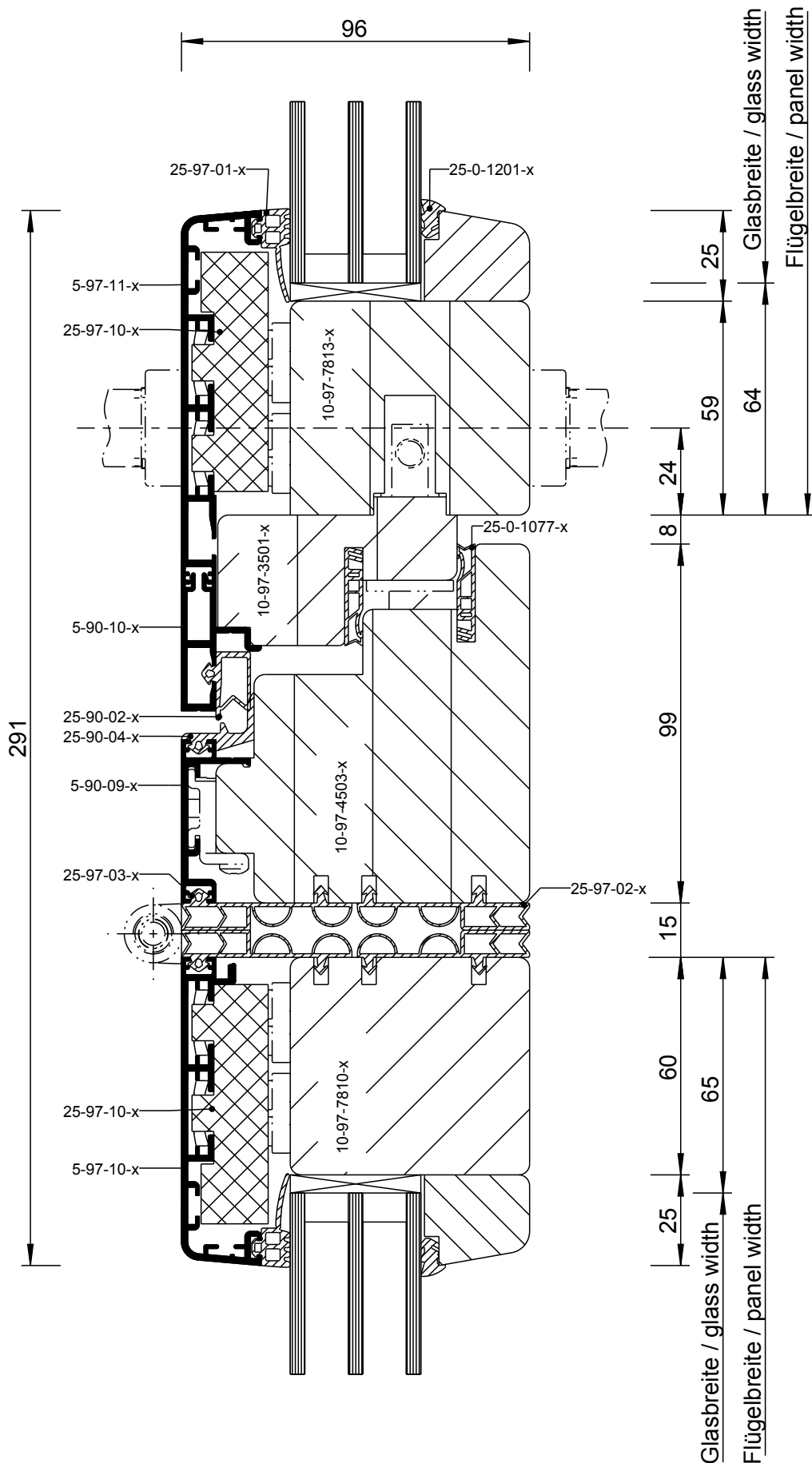
Detail 97-10-3
