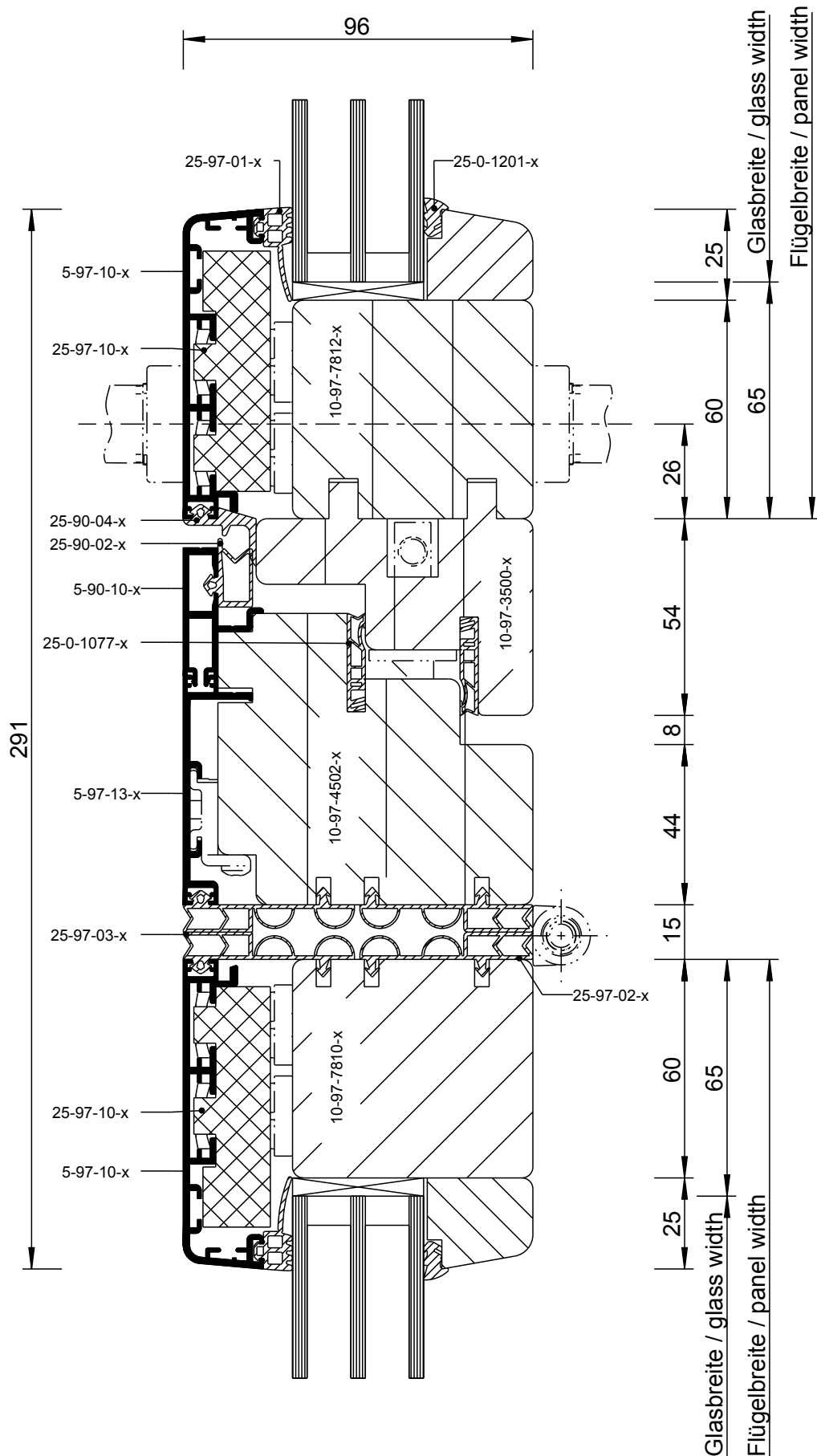
Detail 97-10-2
