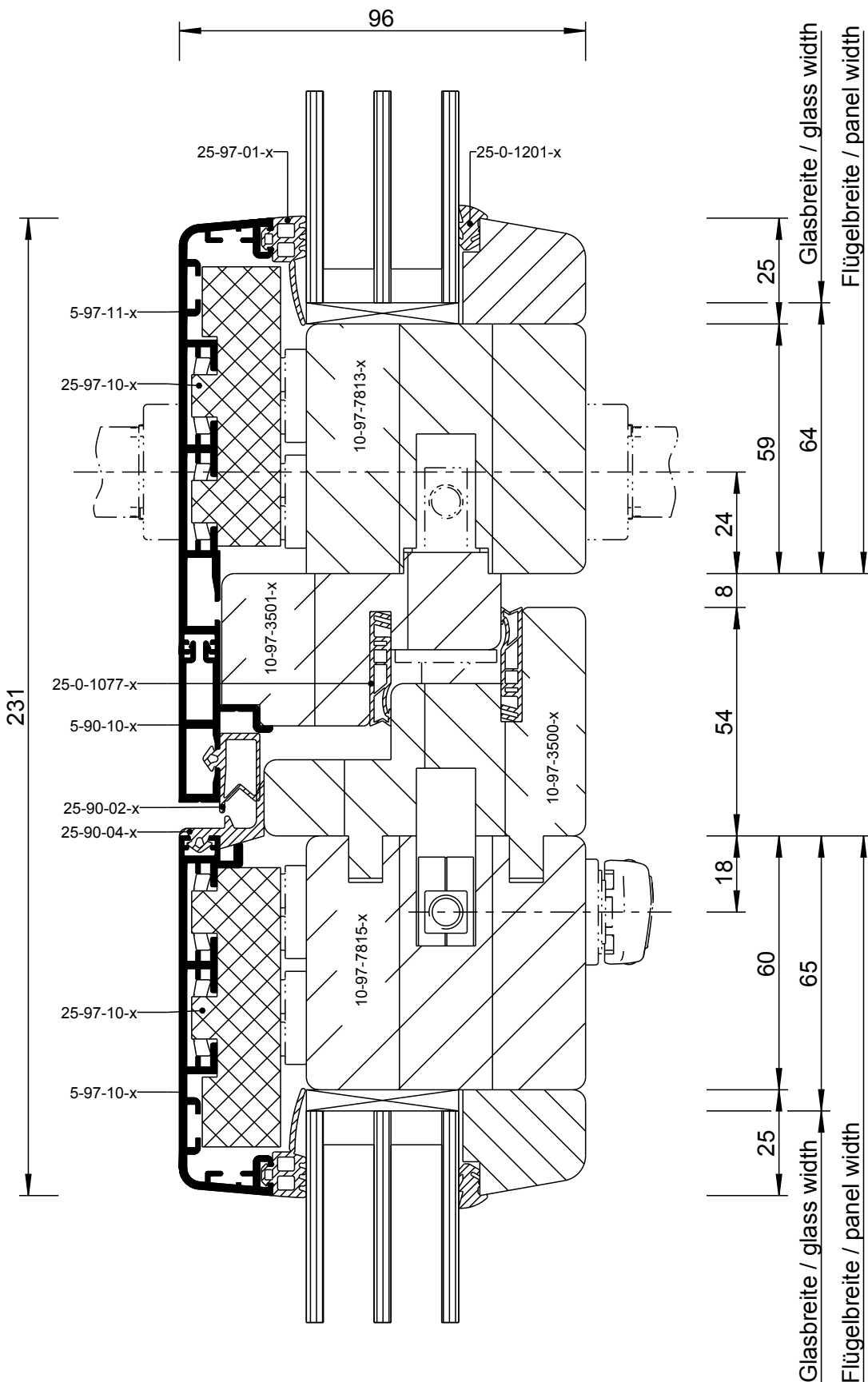
Detail 97-8-3
