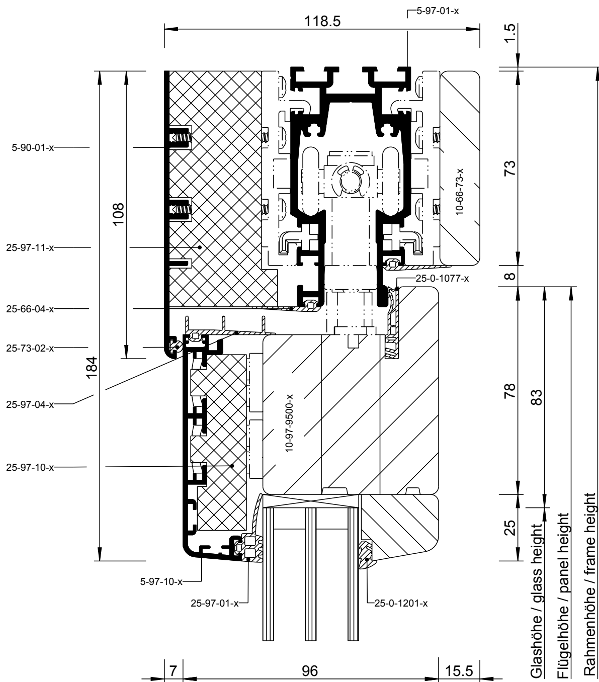
Detail 97-1-2
