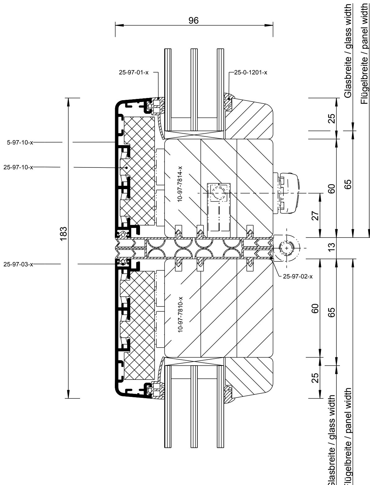
Detail 97-7-3
