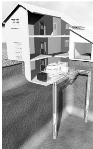
REHAU RAUGEO Probe System
