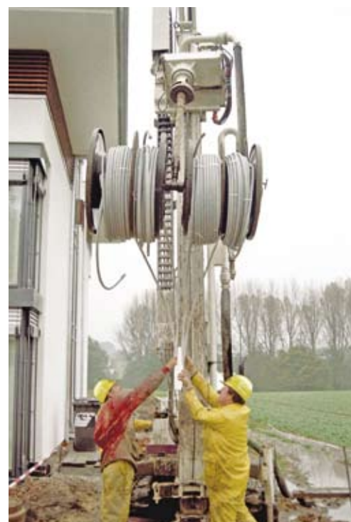
Insertion of PE-Xa Probe
