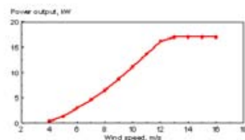
Power output of a 10 m diameter wind turbine
